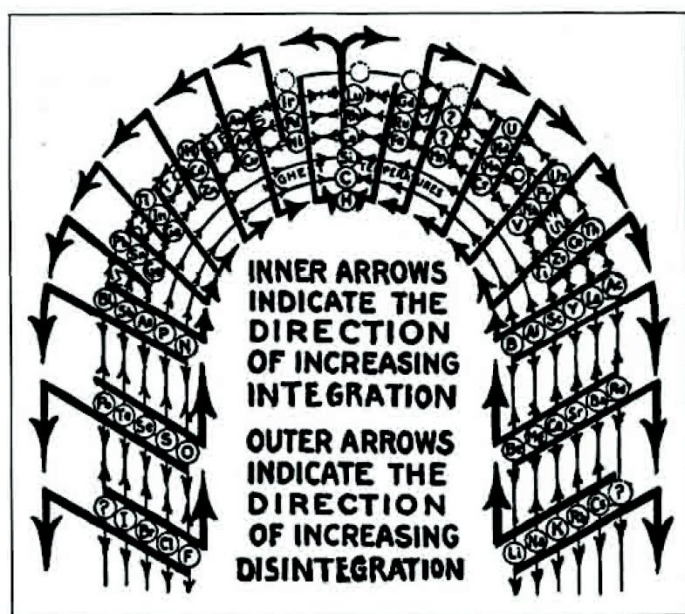
Fig. 77 Opposite actions simultaneously void each other
