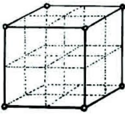
Fig. 5 Mirror planes of reaction
