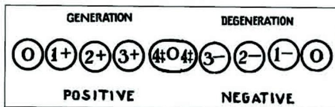
Fig. 68 Two-way journey from zero—through zero—to zero
