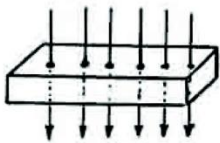
Fig. 42 Light rays are parallel when passing through planes of zero curvature
